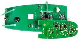
Supported PCB
