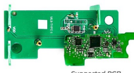
Supported PCB
